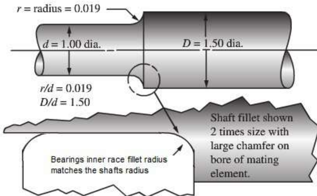
(b) Example of well-rounded fillet ( Larger )
