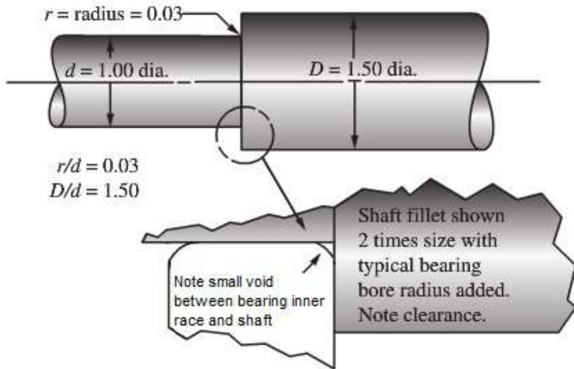
(a) Example of sharp fillet ( Smaller )
