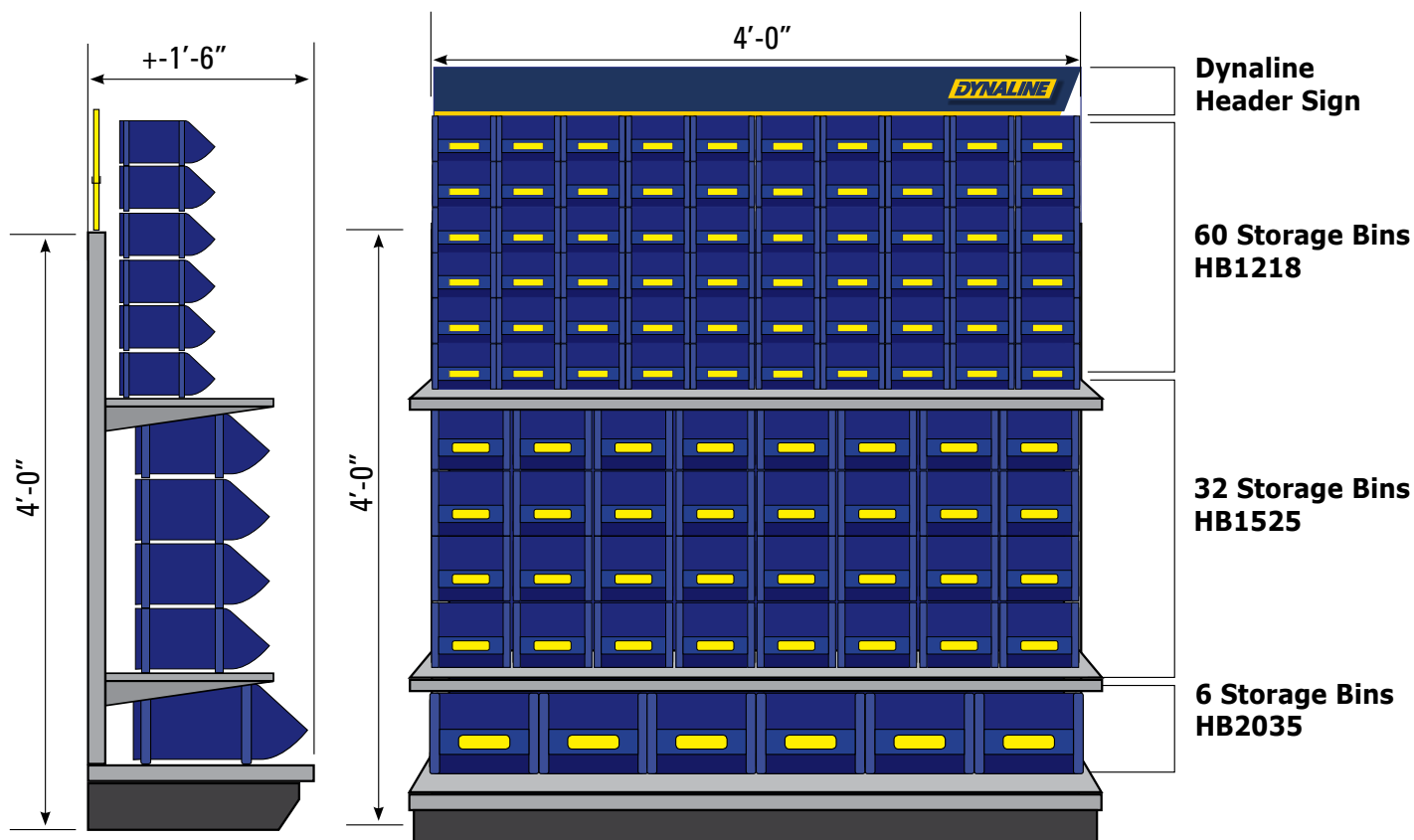
SIDE VIEW
