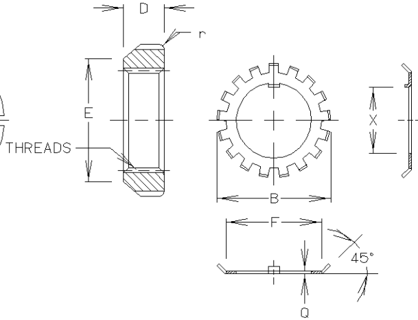
Figure 2 – Lockwashers
