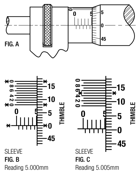
FIGURE C – READING 5.005mm
